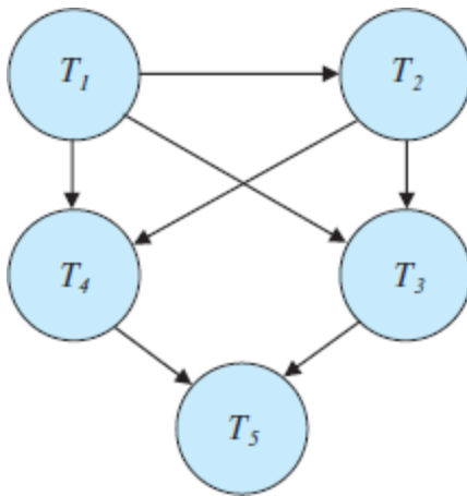
Figure 17.16 Precedence graph for Practice Exercise 17.6 .
