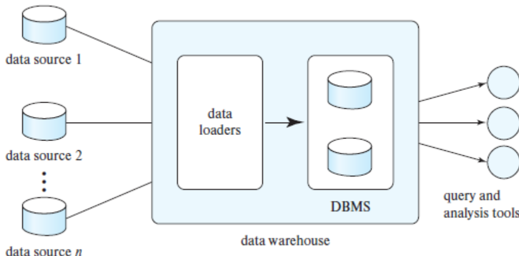
Figure 11.1 Data-warehouse architecture.
